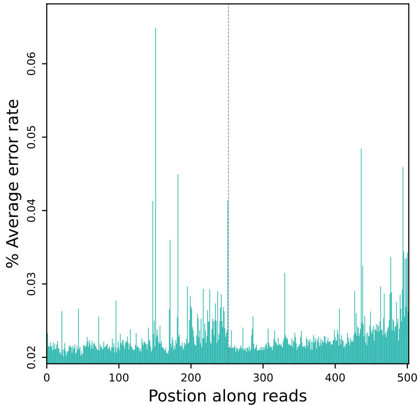
Error rate distribution along reads (R10921)
